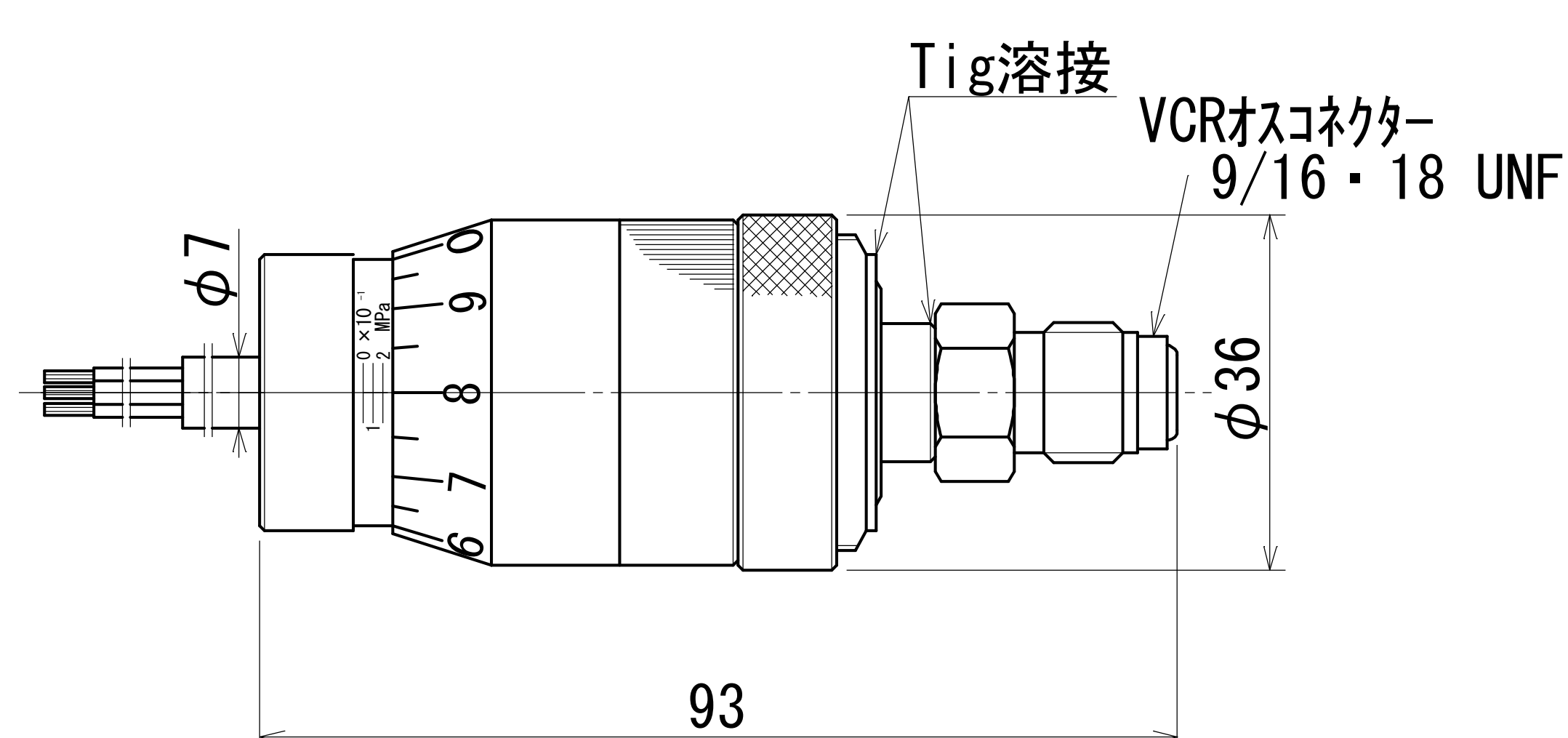
JP-C type
