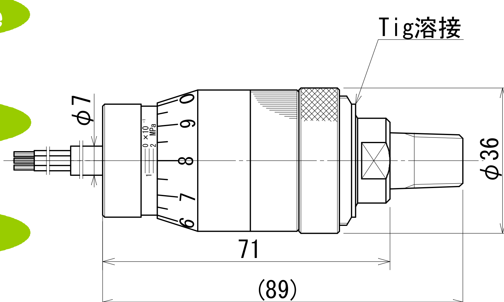
JP-C type
