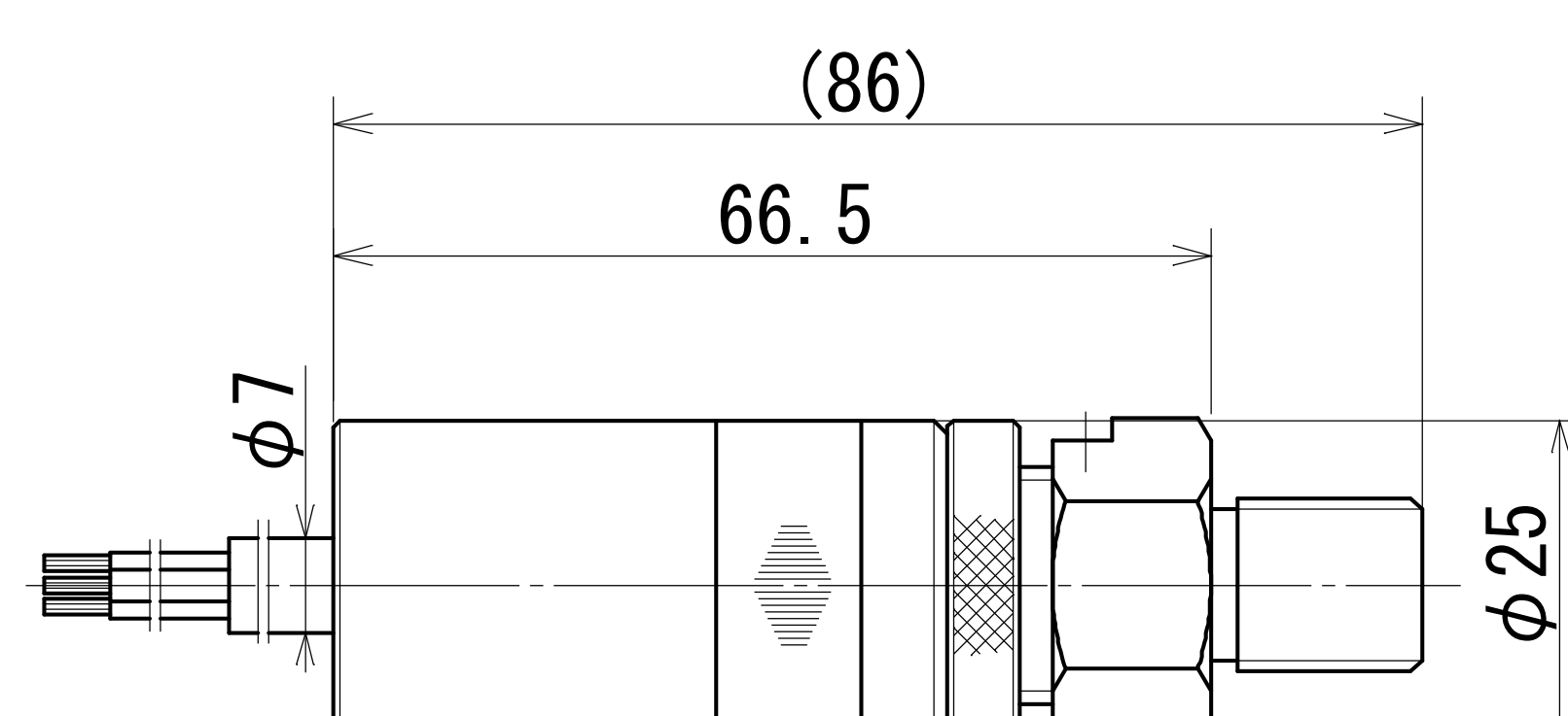
JP-B type
