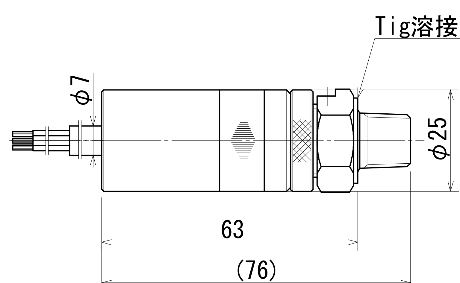
JP-B type
