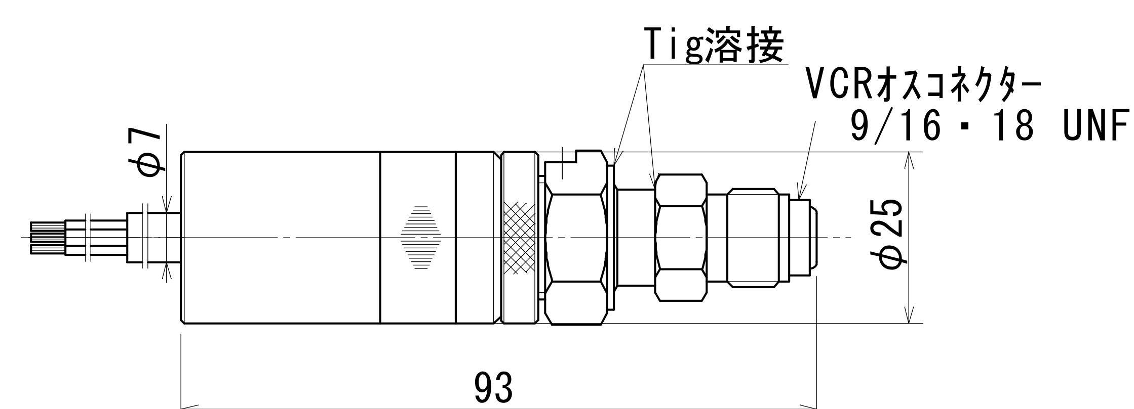
JP-Btype
