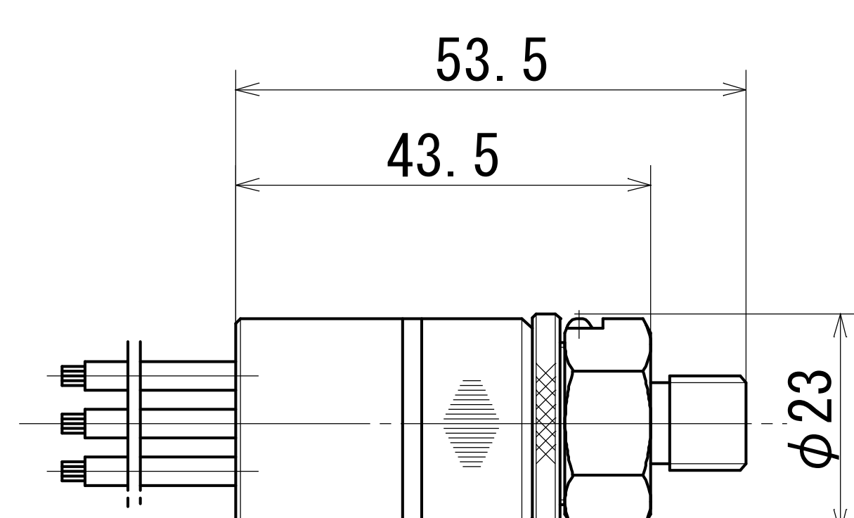
JP-A type
