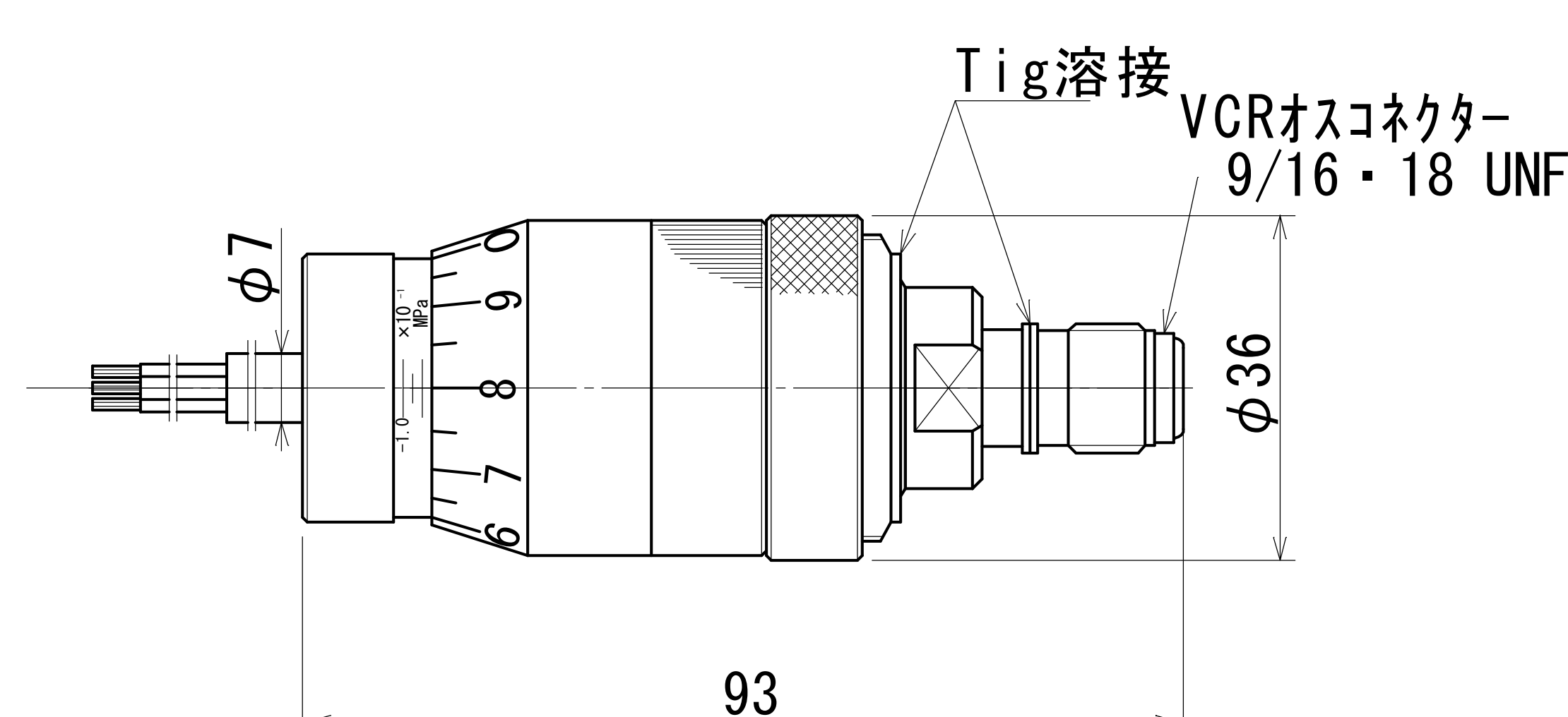
JP-V type
