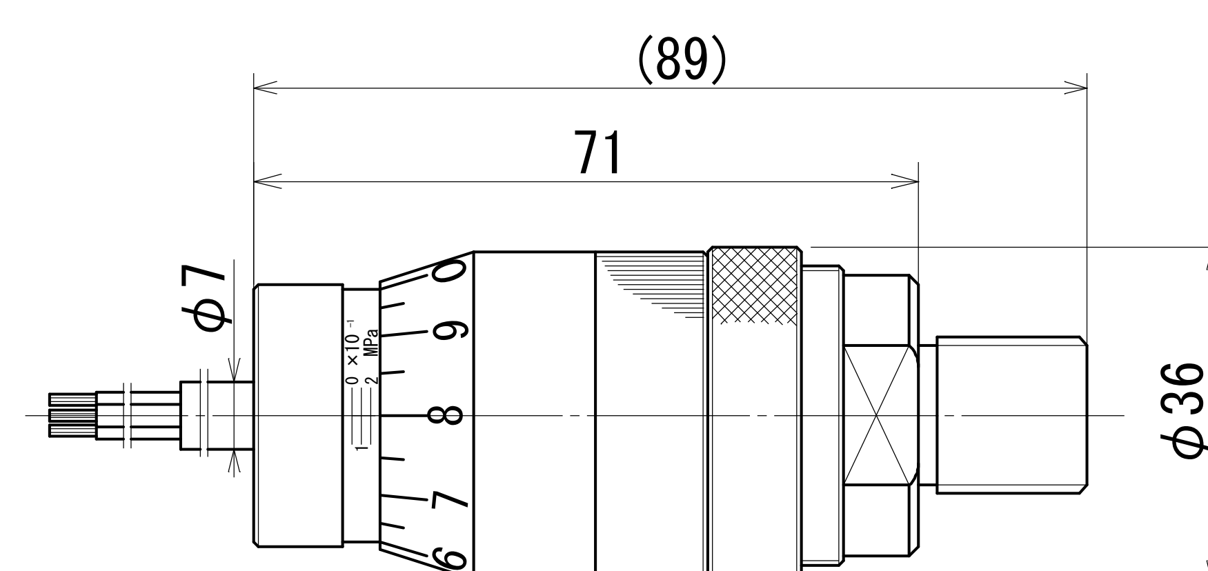
JP-V type
